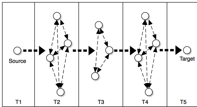
Fig. 2. The first one is a trail with only one broken points. Second is a trail with three continuous broken points. One object first needs to pass all the locations in layer T2 , then T3 and T4 .
